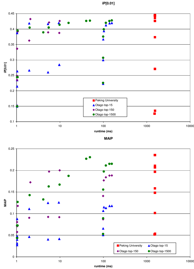
Fig. 3. Trade-off between Effectiveness and Efficiency: iP[0.01] (top) and MAiP (bottom).
