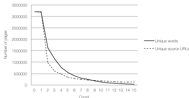
Figure 2: Count of unique source URLs ( dotted line ) and count of unique anchor text words ( solid line ).
